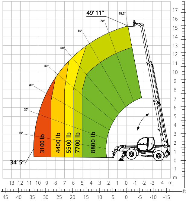
Load chart on stabilizers
