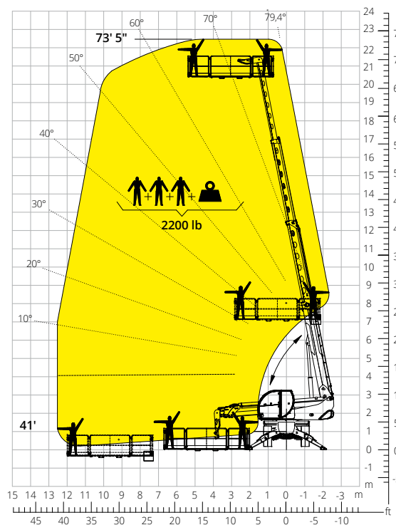
Load chart with ROTATING EXTENDABLE PLATFORM 2,200 lb ATT - 01 - 016
